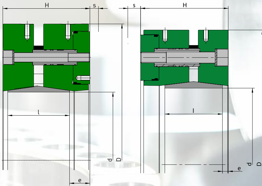
Design with hydraulic system frontside
